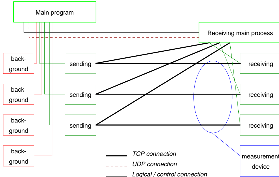
Figure 2 Instrumented kernel measurement system
