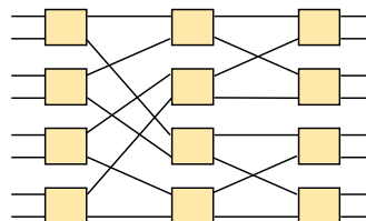
Flip network (inverse shuffle exchange)
