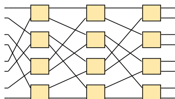
Shuffle exchange (Omega) network
