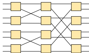
Shuffle exchange (Omega) network
