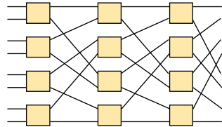
Flip network (inverse shuffle exchange)
