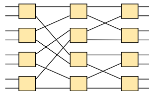
Flip network (inverse shuffle exchange)
