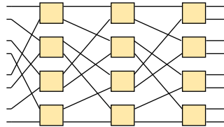
Shuffle exchange (Omega) network
